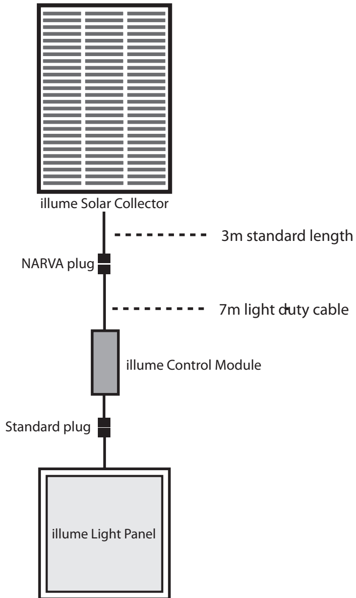
Example of illum Premium Connection System
