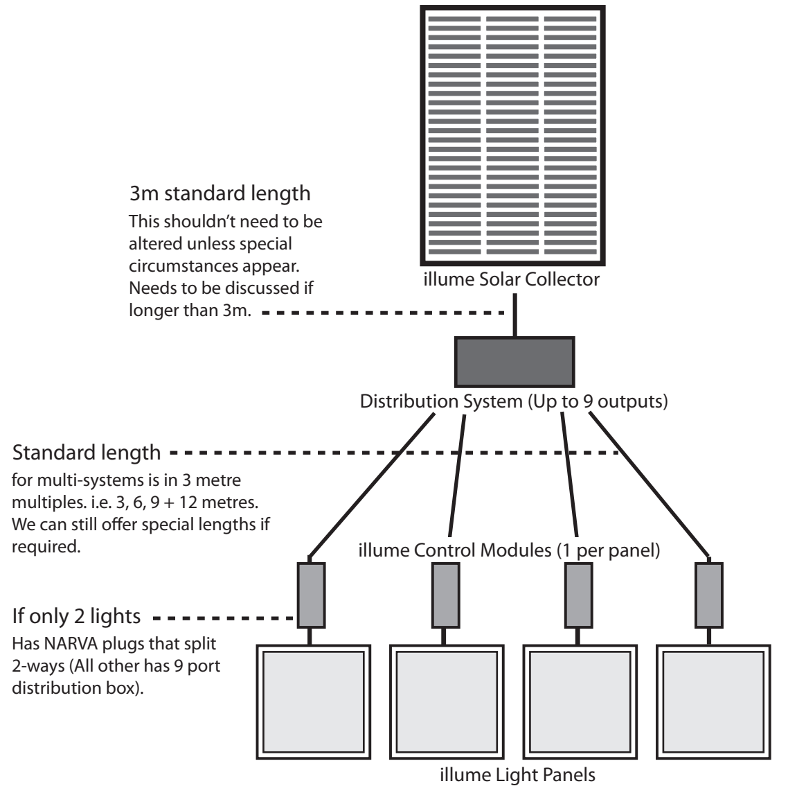
Example of illum Premium Multiple Unit System (4x unit eg.)
